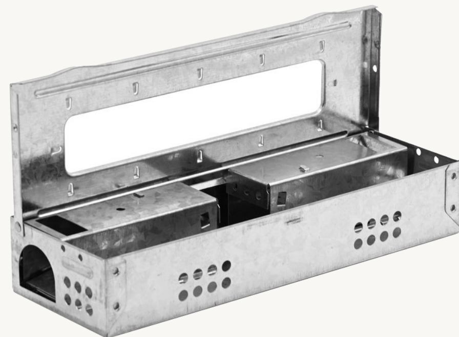
OPEN PRODUCT VIEW / NARROW BODY + TWO ENCLOSED END TUNNELS
